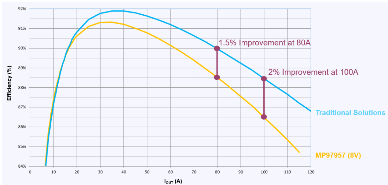
Figure 2: 16V vs. 8V Efficiency Comparison
