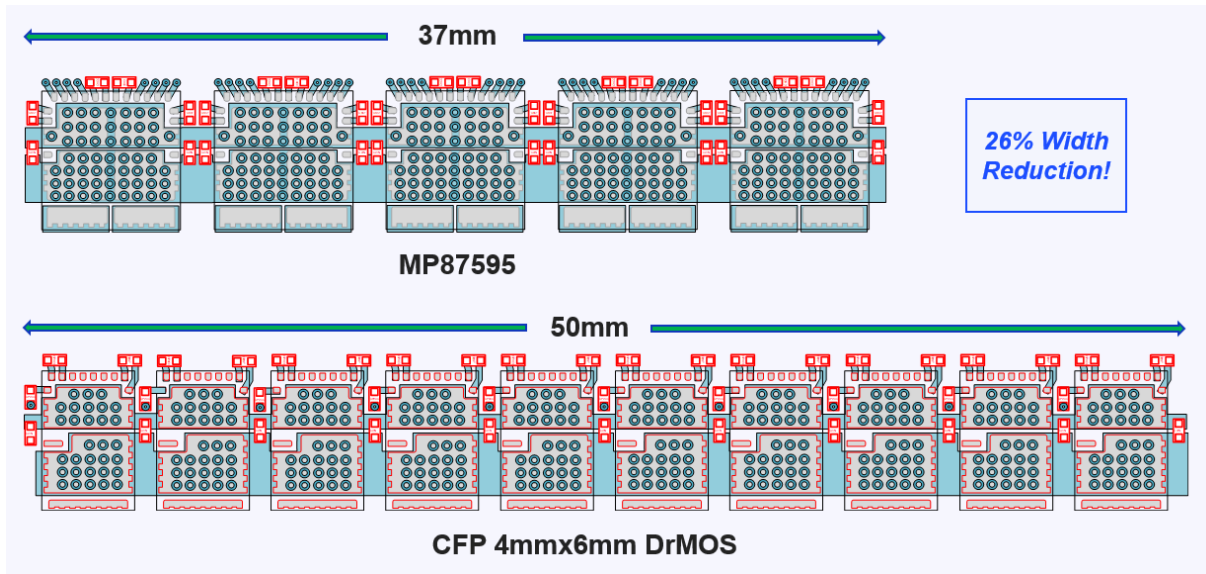
Figure 1: High Power Density in Compact PCB Space
