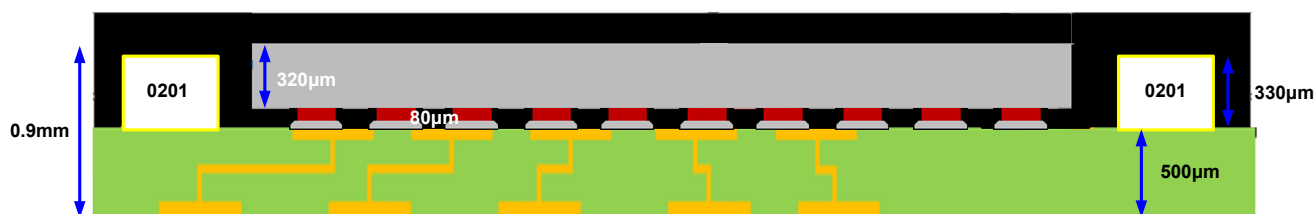
Figure 4: Overmolded Top Package Option
