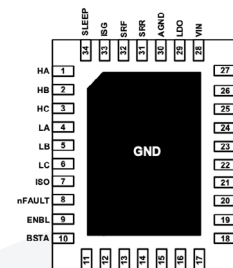
MP6633A – QFN-34 (4mmx5mm)
