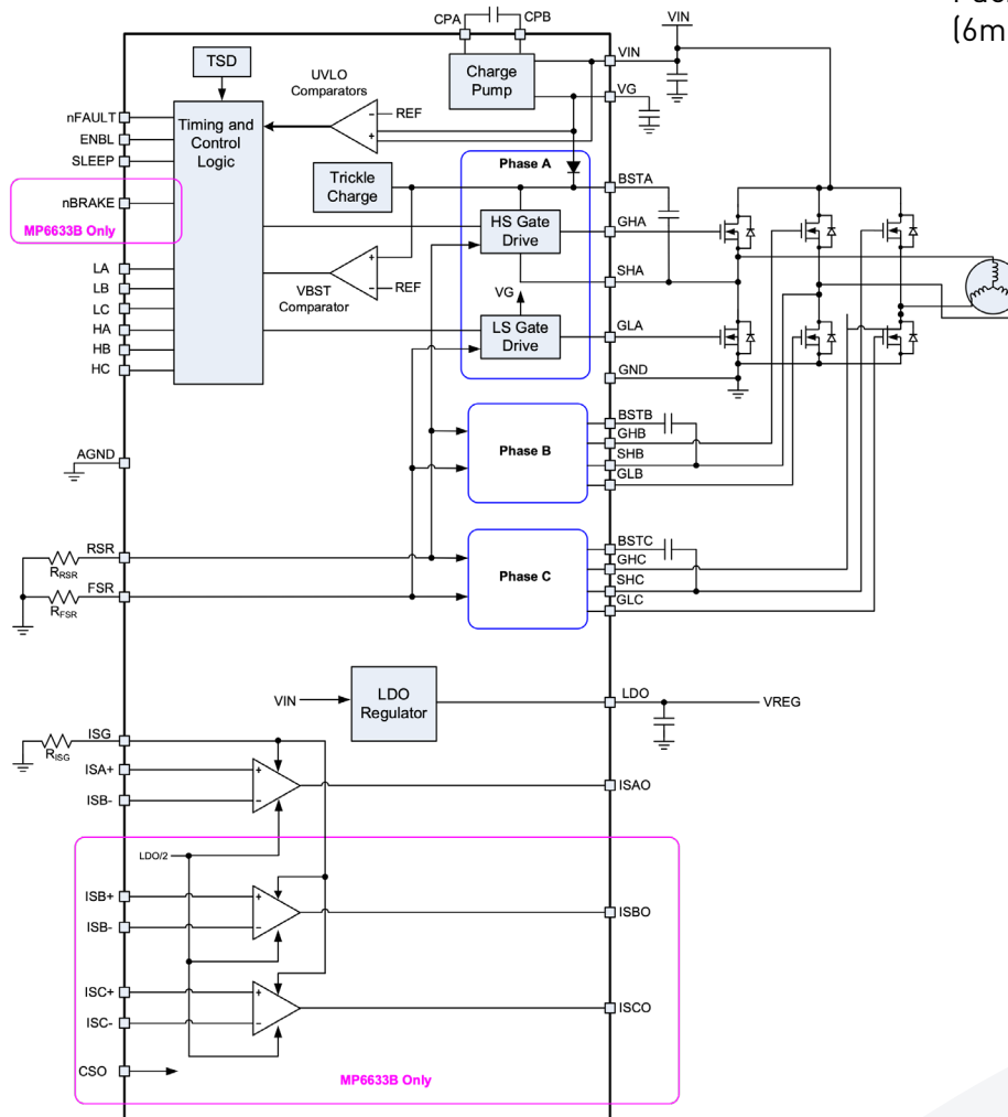
MPQ6633B – QFN-48 (6mmx6mm)
