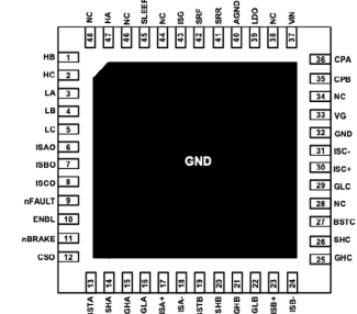
MPQ6633B – QFN-48 (6mmx6mm)
