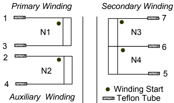
Pin Definition of Bobbin
