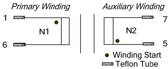
Pin Definition of Bobbin
