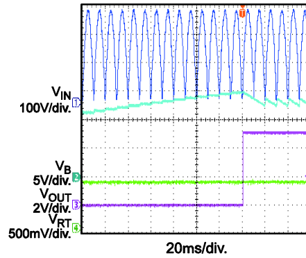
RT Protection Recovery 230Vac
