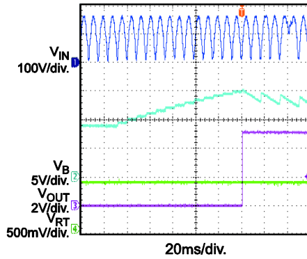
RT Protection Recovery 115Vac
