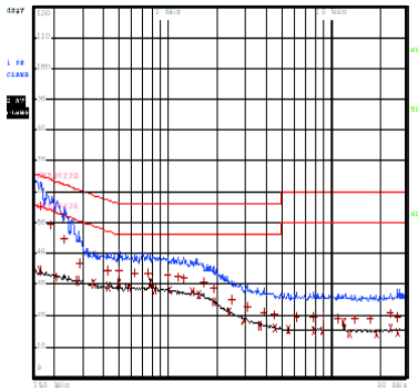
EMI Performance 115Vac, N Line
