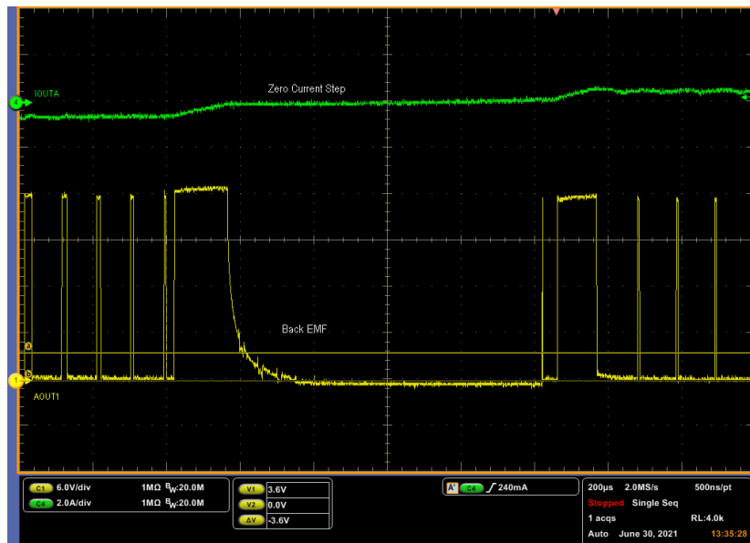
Figure 7: Stalled Motor
