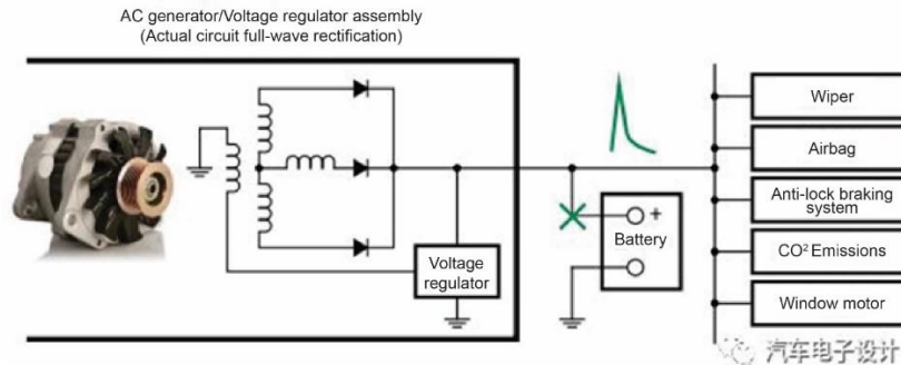
Most of the transient in a vehicle's electrical system are caused by AC generators
